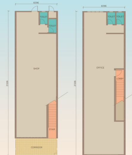
INTERMEDIATE UNIT - TYPE A GROUND FLOOR PLAN SCALE 1: 100
